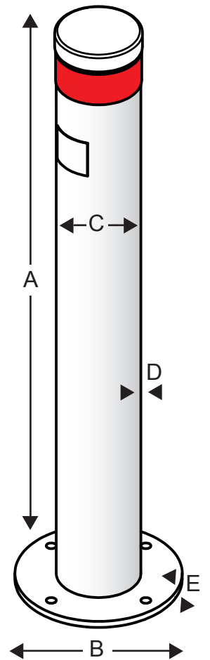
Dugite (Surface Mount) Bollard
