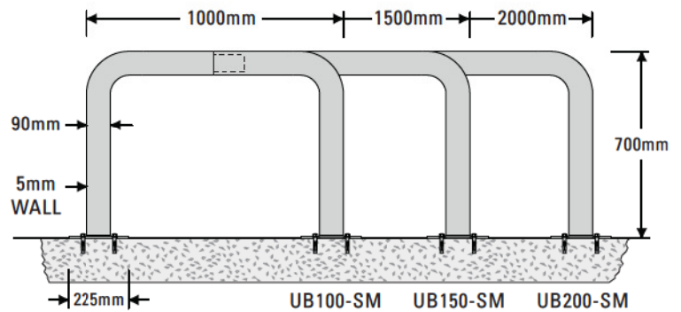
SURFACE MOUNT MODEL (Front view)
